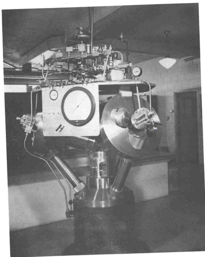
Figure - 2 Tetrahedral Anvil Press
